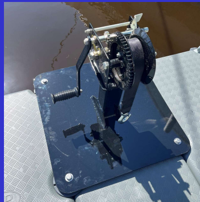
Heavy Duty Two Speed Winch Powder Coated For Corrosion Protection
